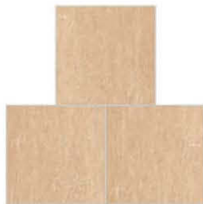
Random Phases
